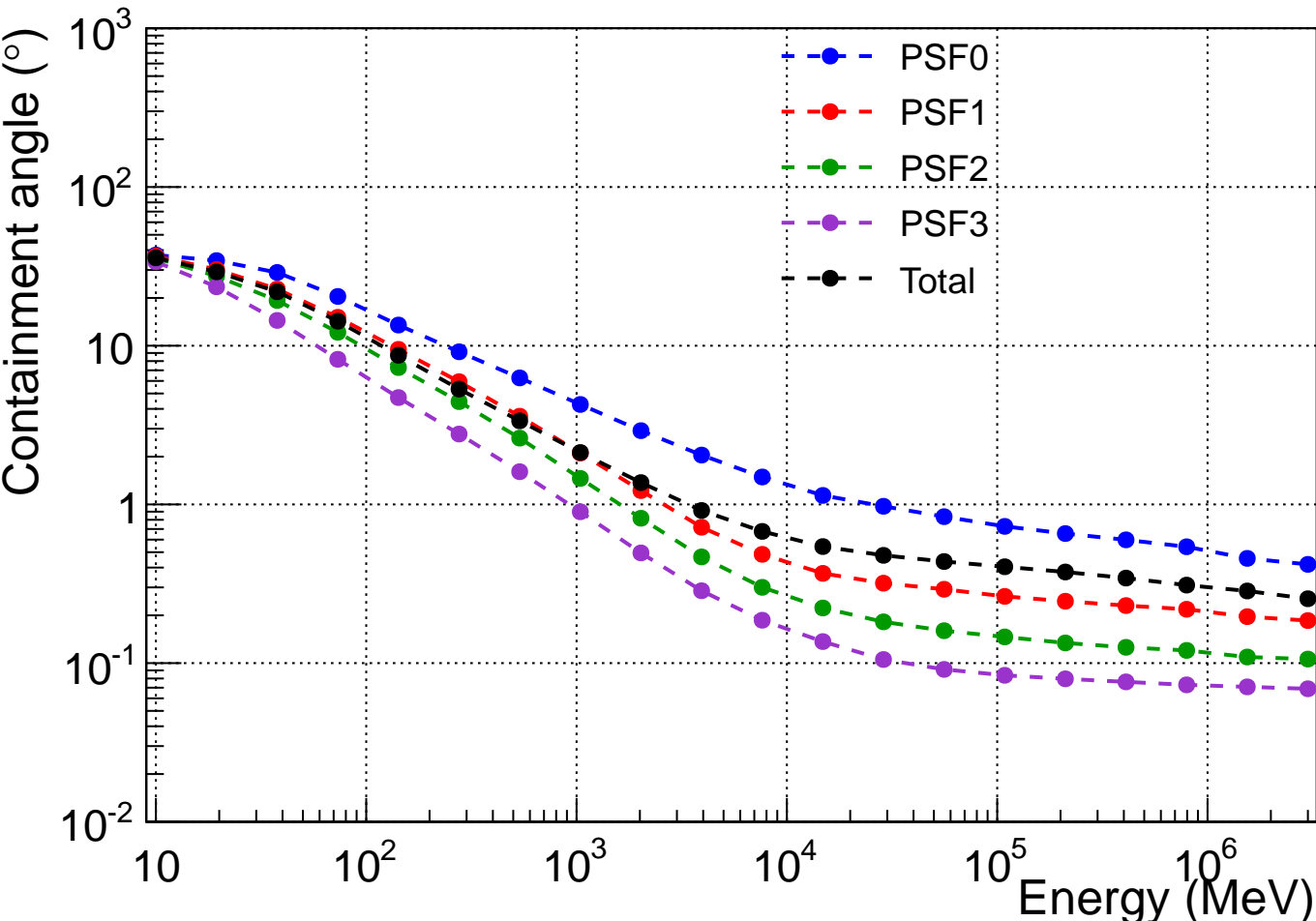
P8R2_SOURCE_V6 PSF at normal incidence 95% containment
