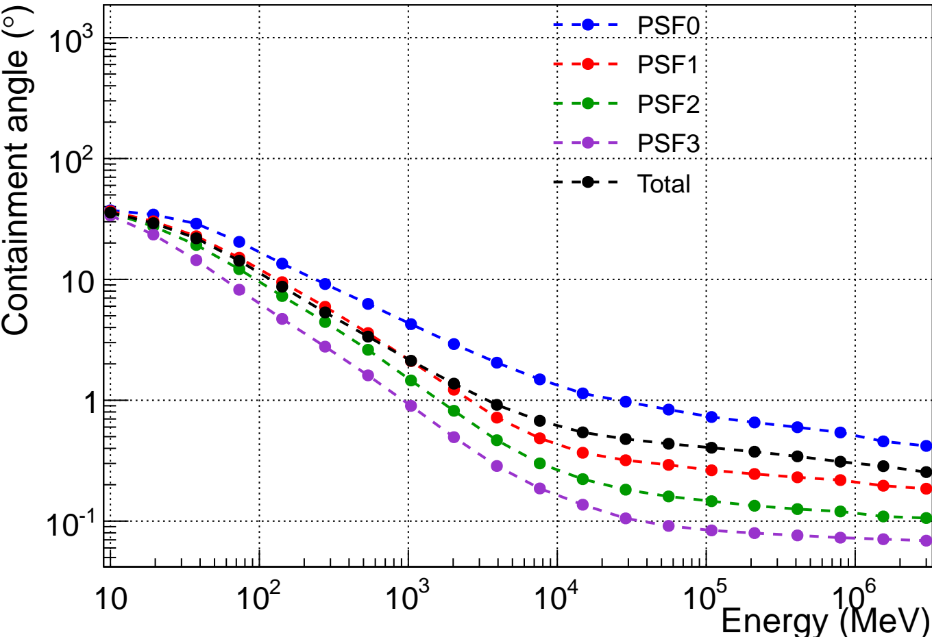
P8R2_SOURCE_V6 PSF at normal incidence 95% containment
