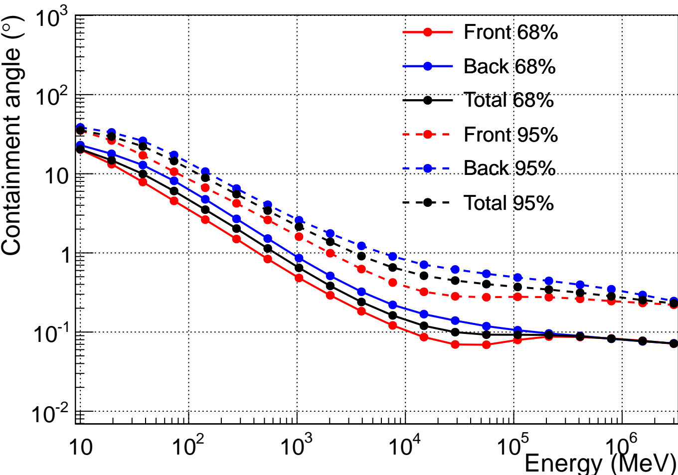
P8R2_SOURCE_V6 PSF at normal incidence
