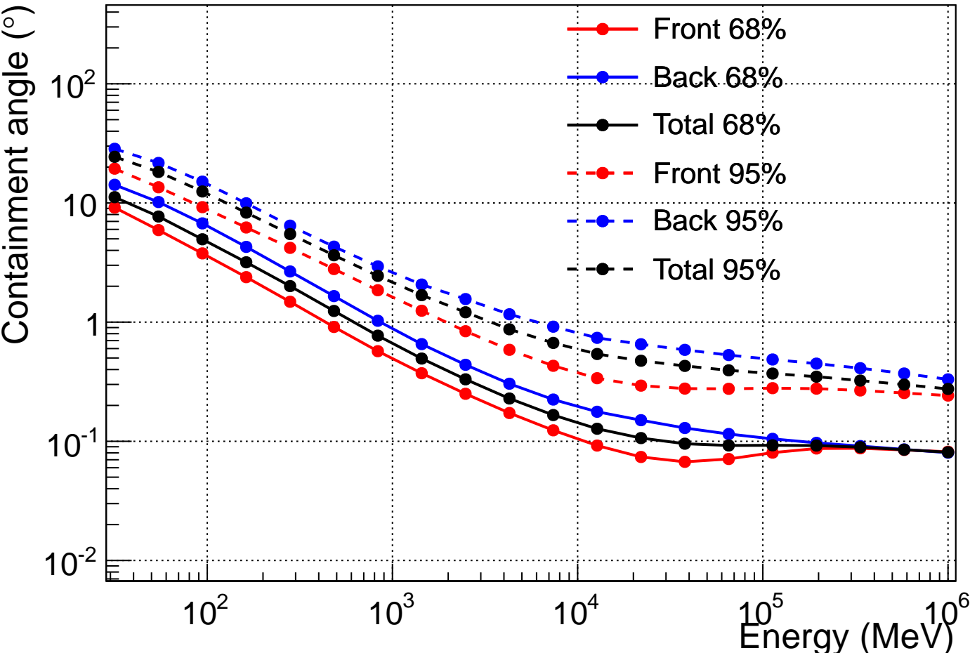
P8R2_SOURCE_V6 PSF at normal incidence
