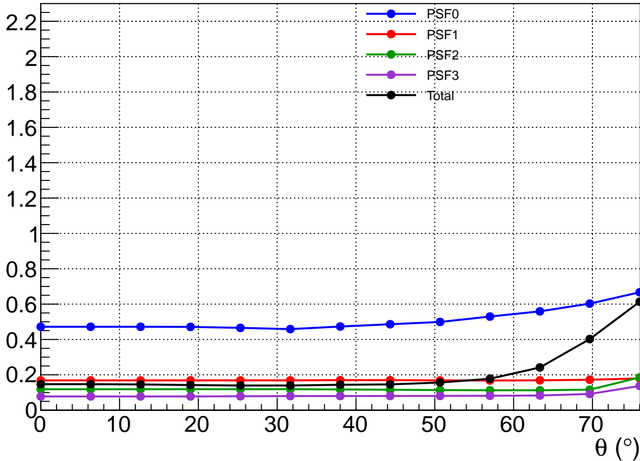
P8R2_SOURCE_V6 PSF at 10 GeV 68% containment
