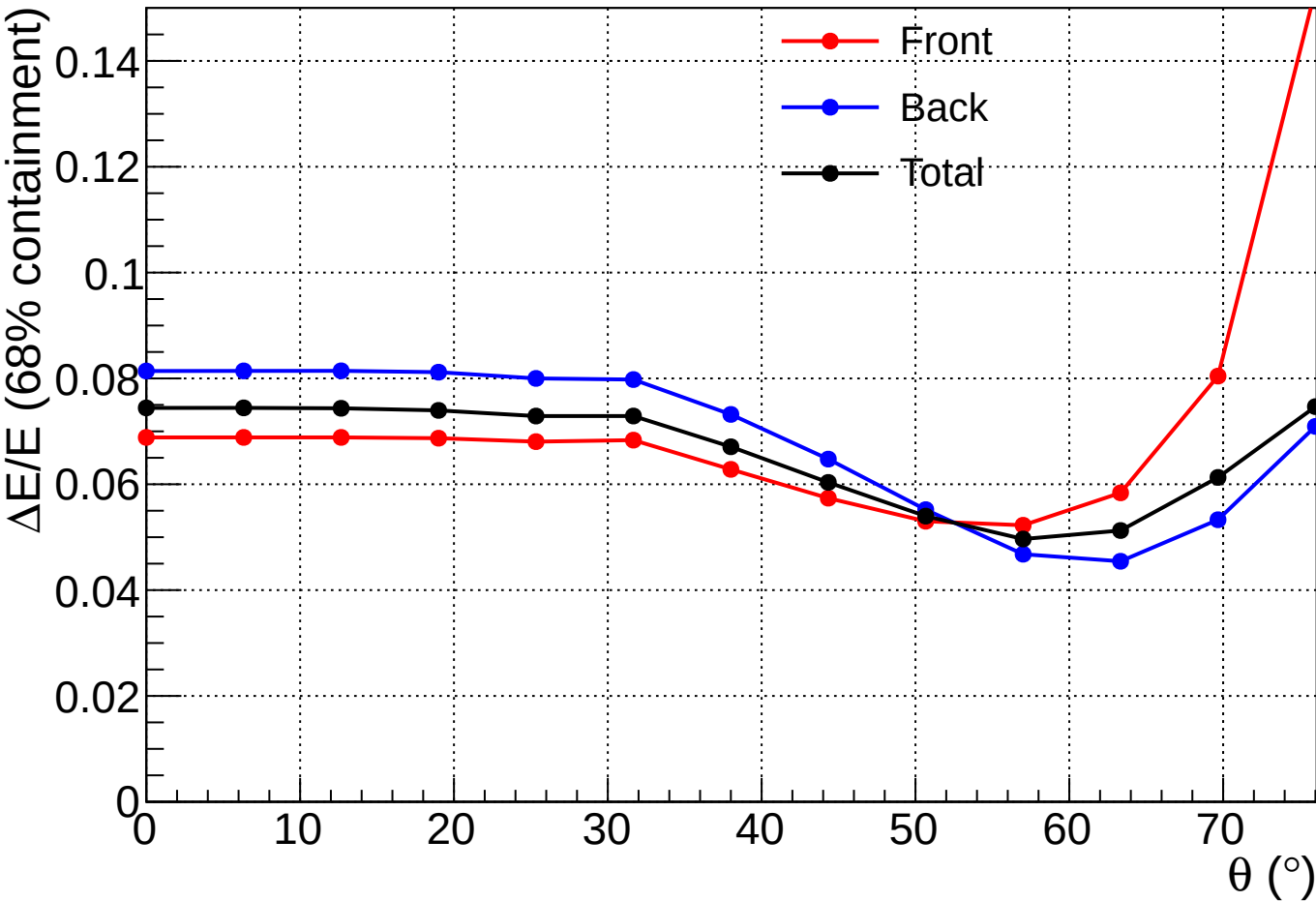
P8R2_SOURCE_V6 energy resolution at 10 GeV
