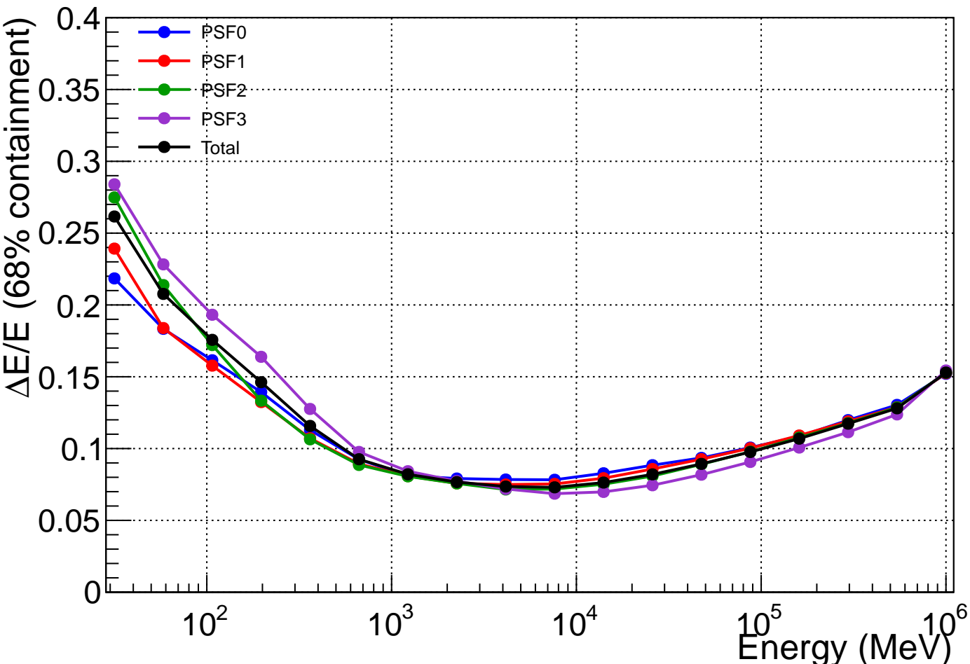
P8R2_SOURCE_V6 energy resolution at normal incidence
