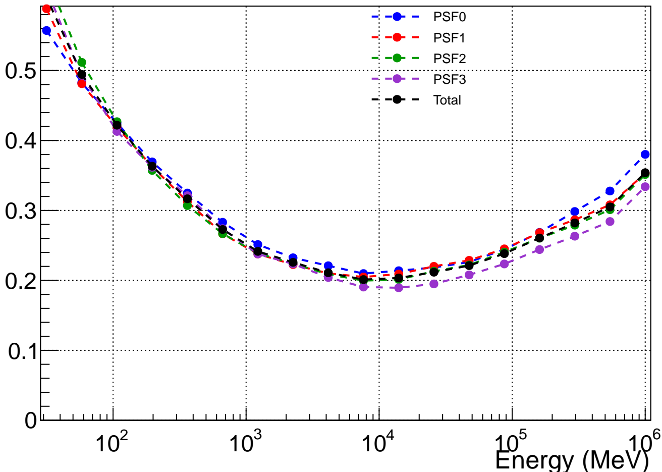
P8R2_SOURCE_V6 theta-average Edisp 95% containment
