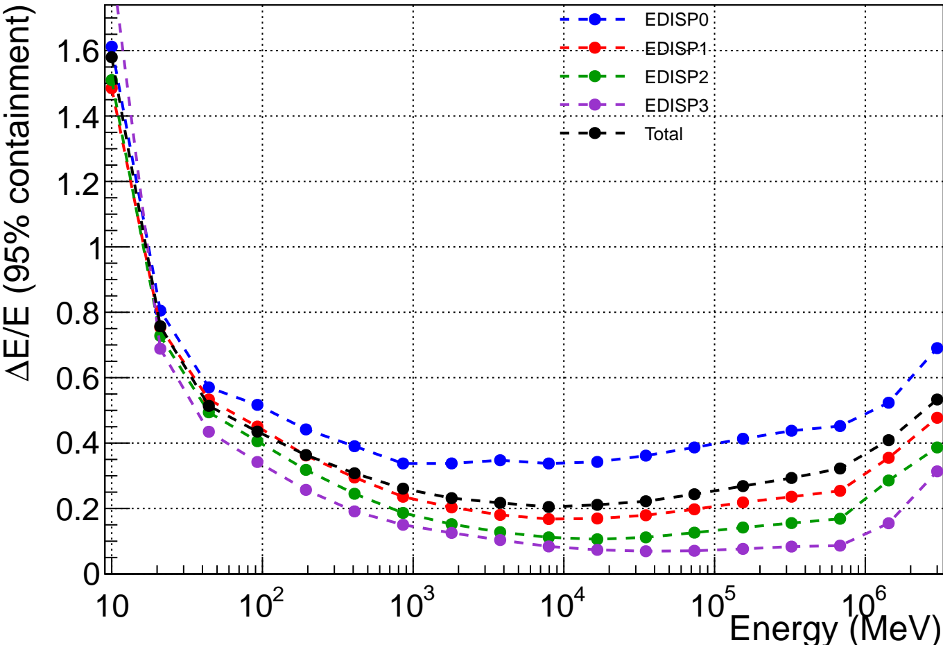
P8R2_SOURCE_V6 theta-averaged energy resolution 95% containment
