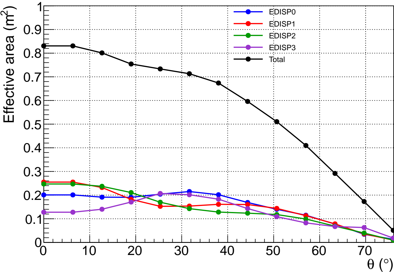
P8R2_SOURCE_V6 effective area at 1 GeV, averaged over \phi
