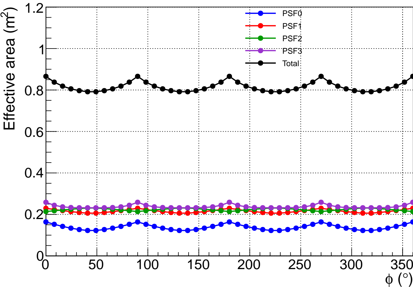
P8R2_SOURCE_V6 effective area at 10 GeV, \theta = 30^\circ
