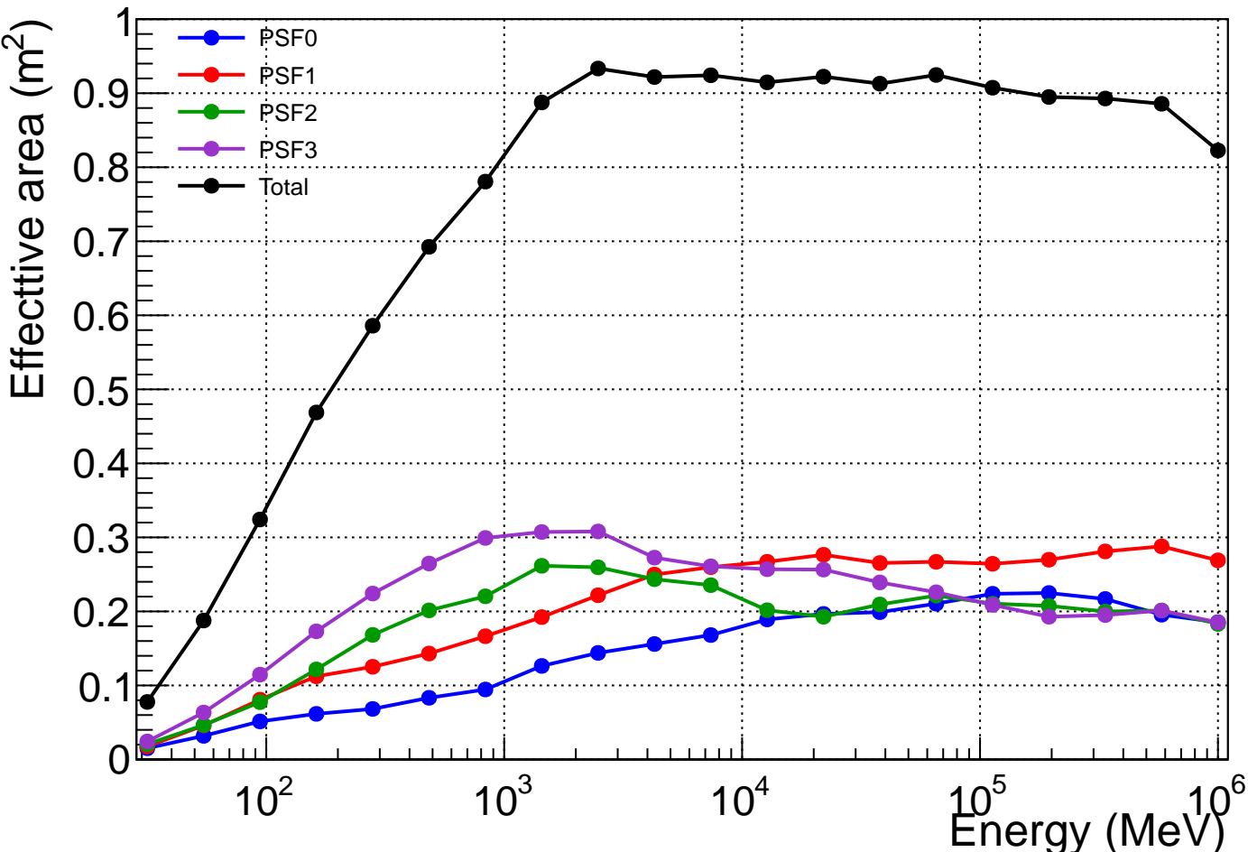
P8R2_SOURCE_V6 effective area at normal incidence ( \cos(\theta) > 0.975 )
