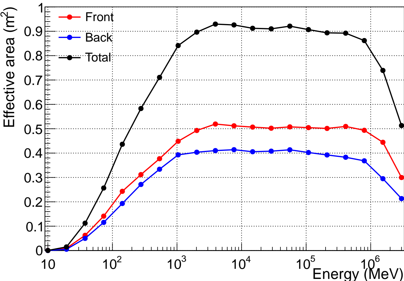
P8R2_SOURCE_V6 on-axis effective area
