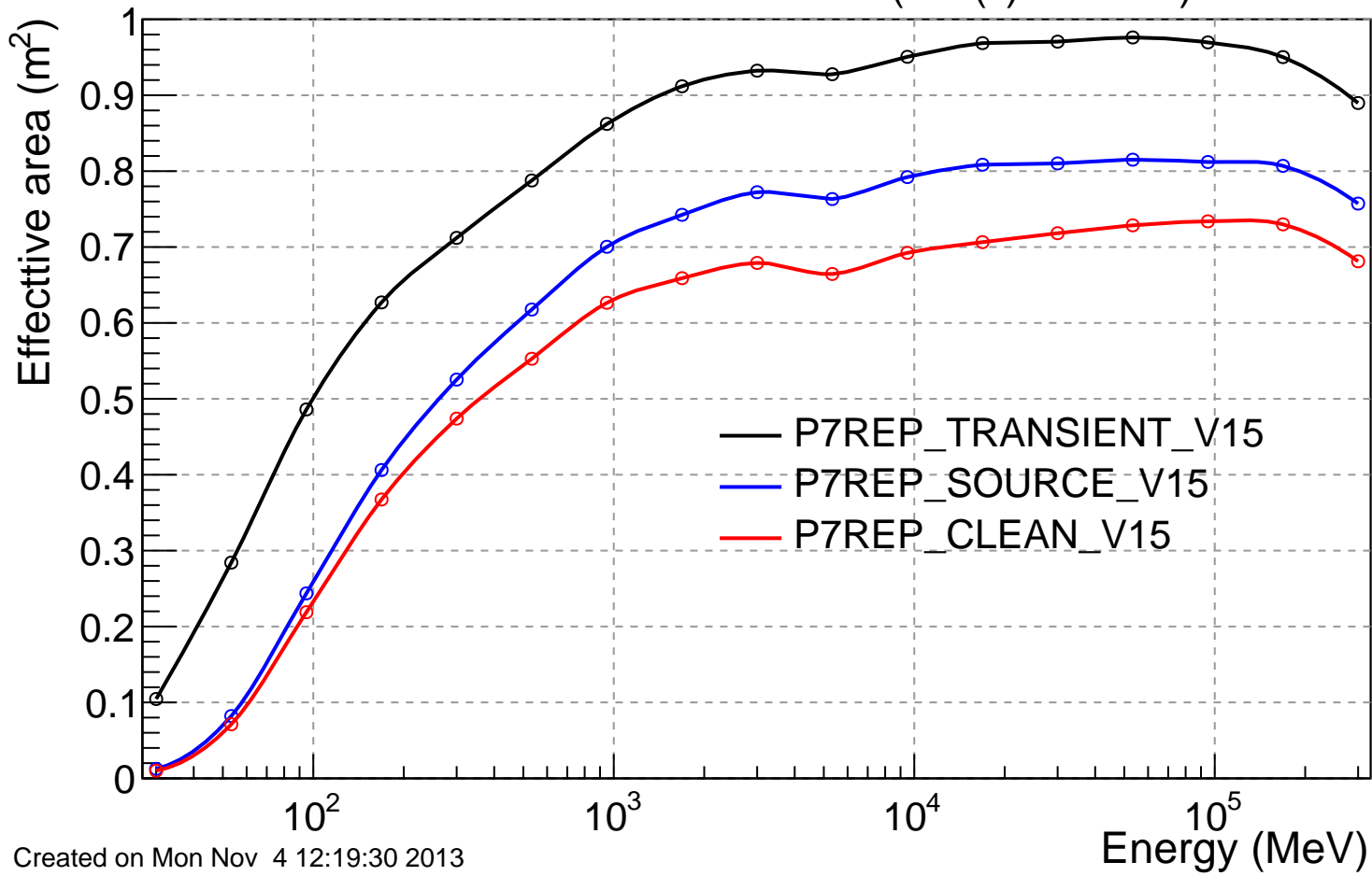
Effective area at normal incidence ( \cos(\theta) > 0.975 )
