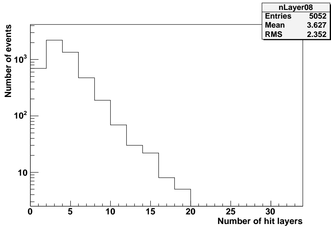
Figure 4: Number of hit layers in tower 08
