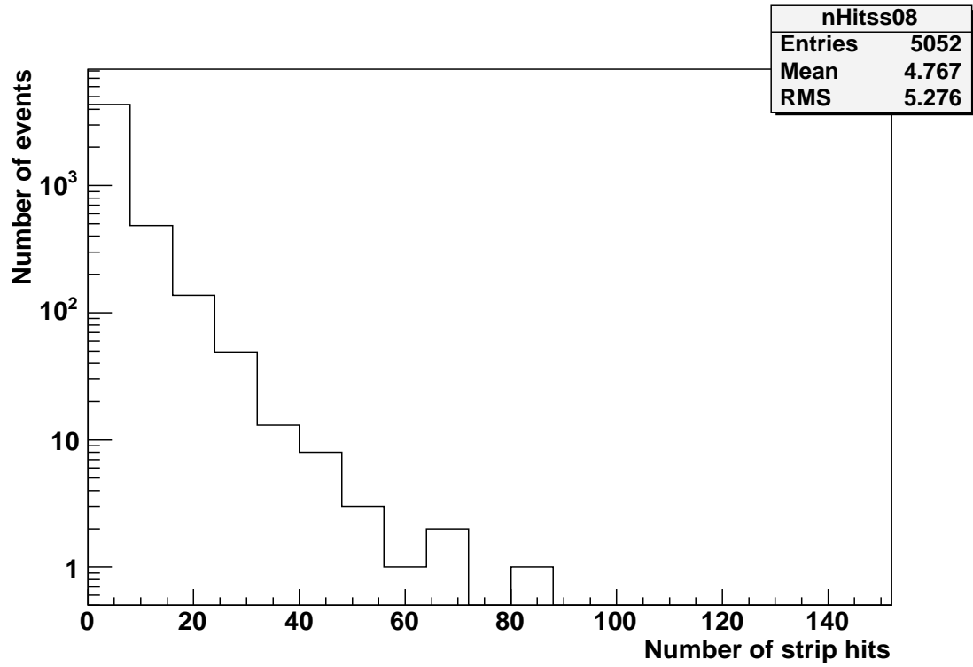
Figure 2: Number of hit strips in tower 08
