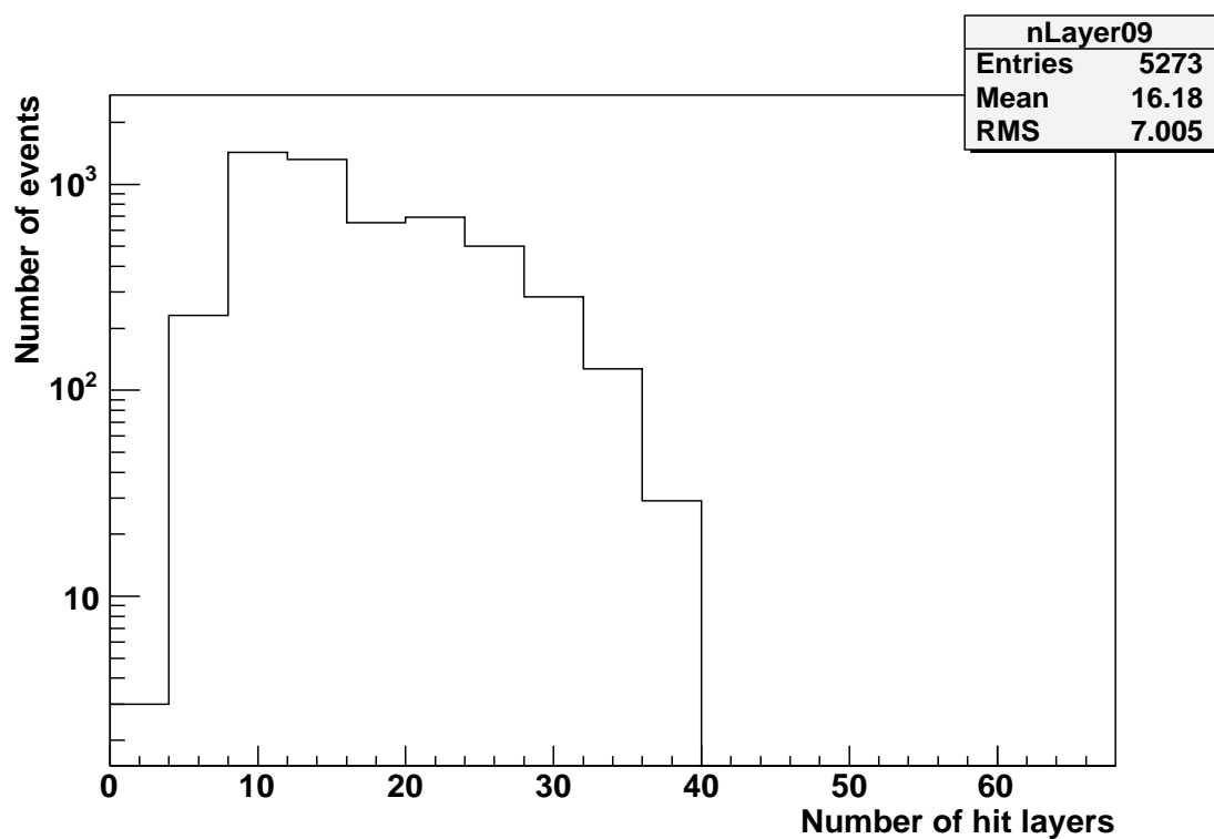
Figure 5: Number of hit layers in tower 09
