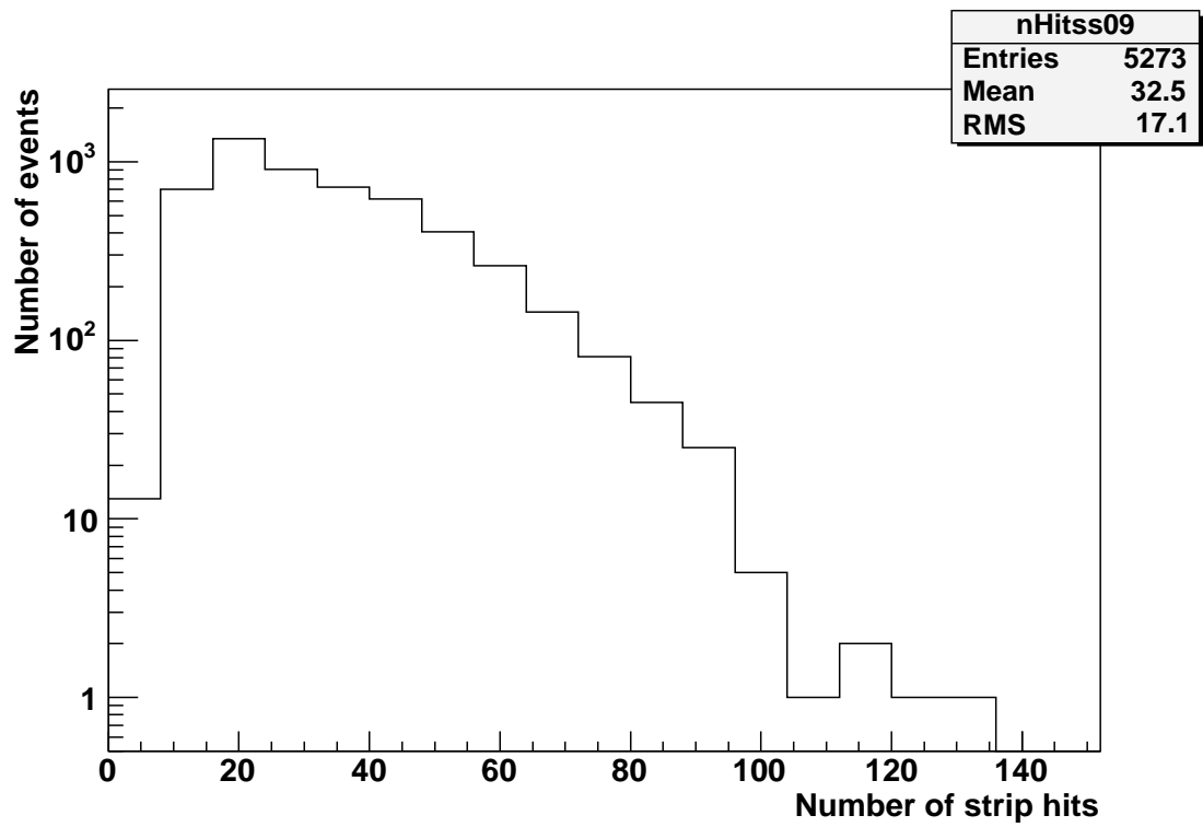
Figure 3: Number of hit strips in tower 09
