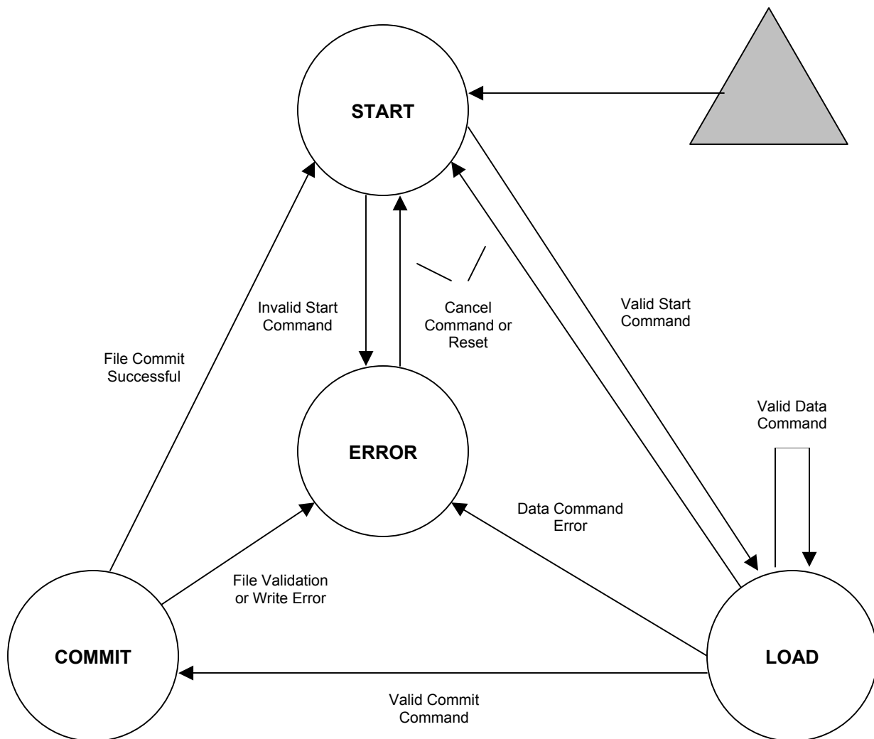
Figure 4 - File Upload State Diagram
