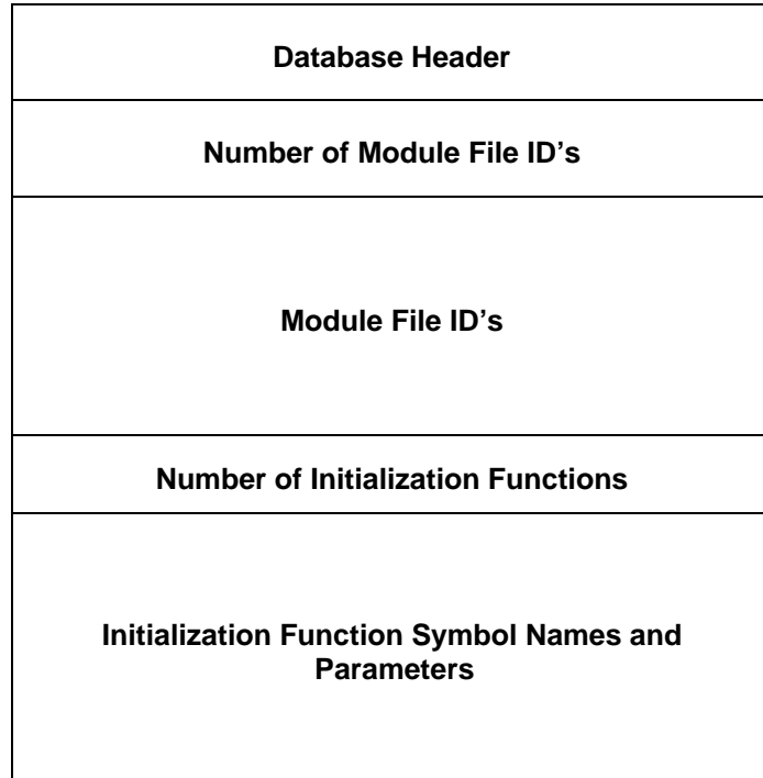
Figure 9 - Application Database File Format
