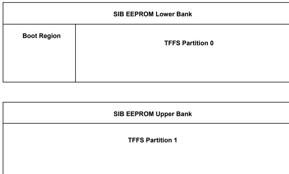
Figure 4 - SIB EEPROM Layout
