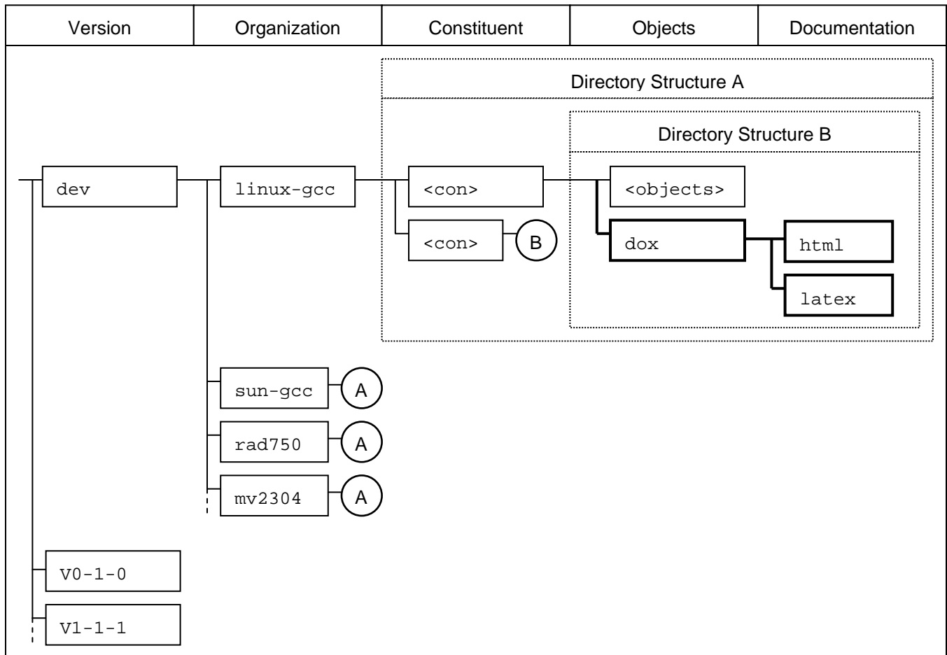
Figure 28 Public directory structure extensions for Doxygen
