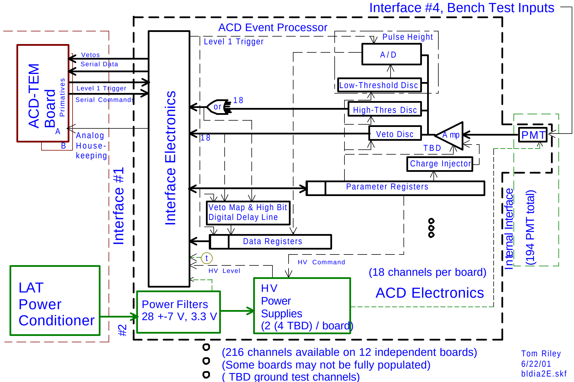
Fig 4.2-1 GLAST ACD Electronic Functional Block Diagram Level 2, ACD Electronics
