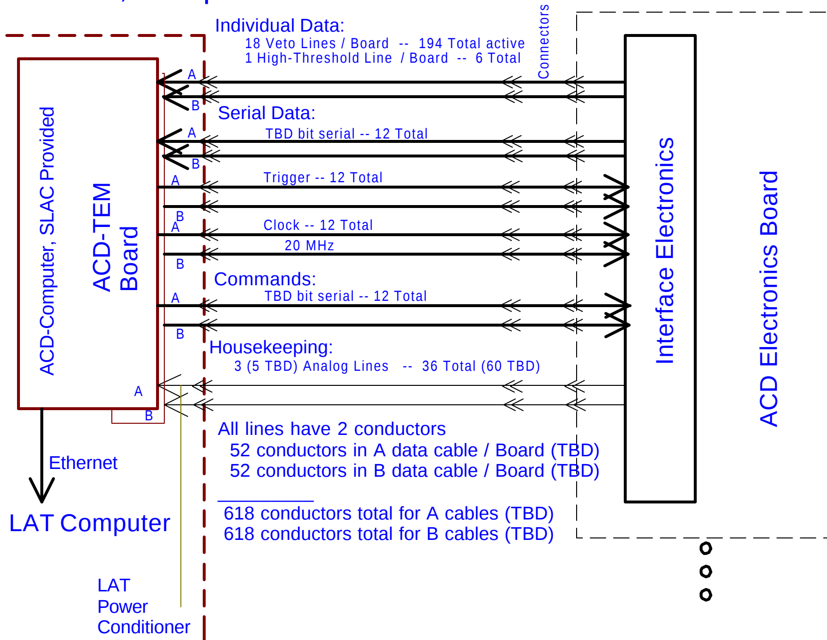
Fig 4.3-1 GLAST ACD Electronic Functional Block Diagram Level 2, Computer Interface
