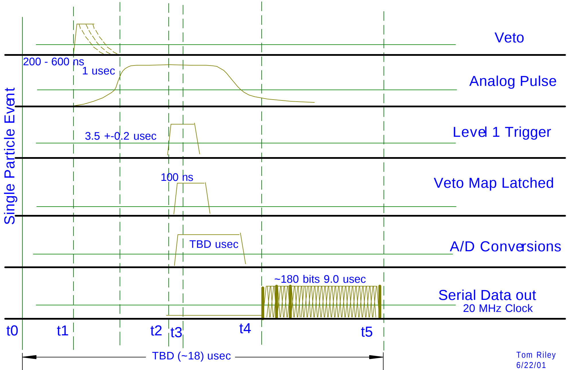
Fig 5.4.1.4-1 GLAST ACD Electronic to ACD-TEM Timing Diagram
