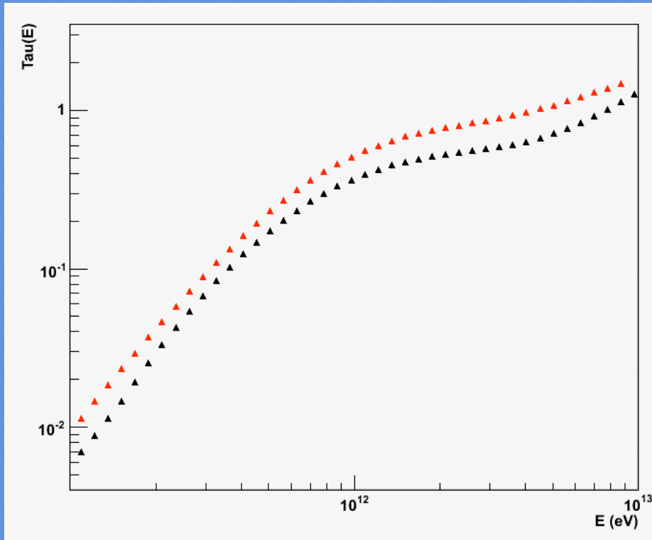
Optical Depth
