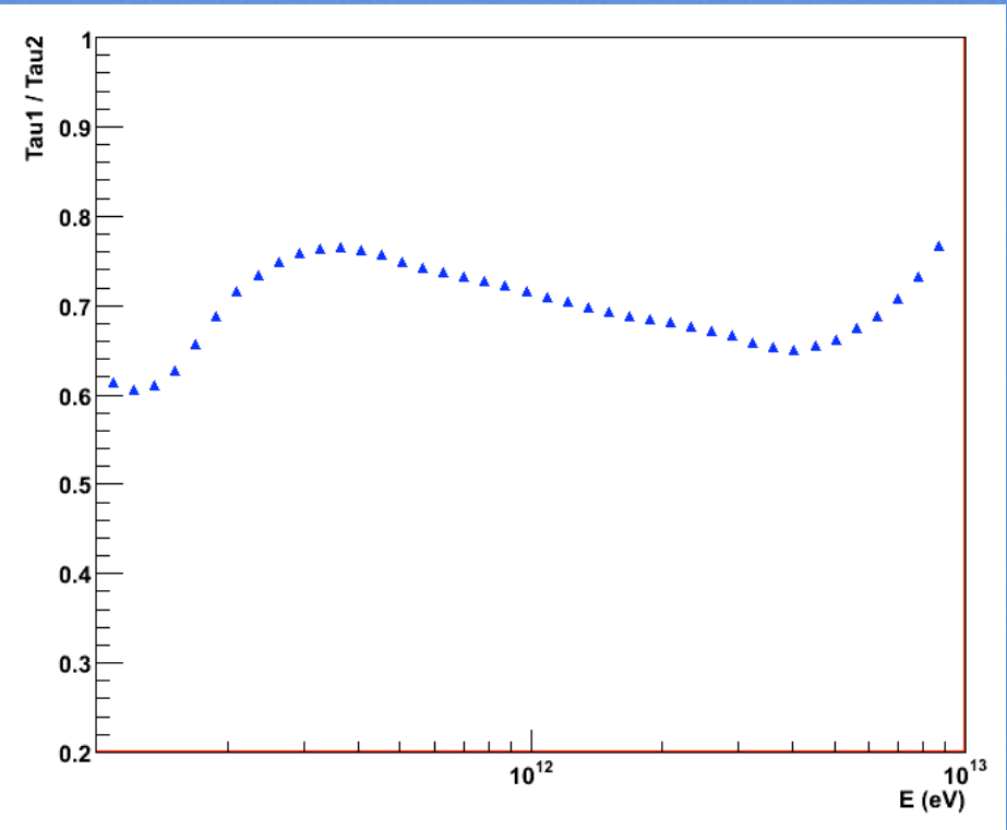
Ratio Kneiske / Franceschini
