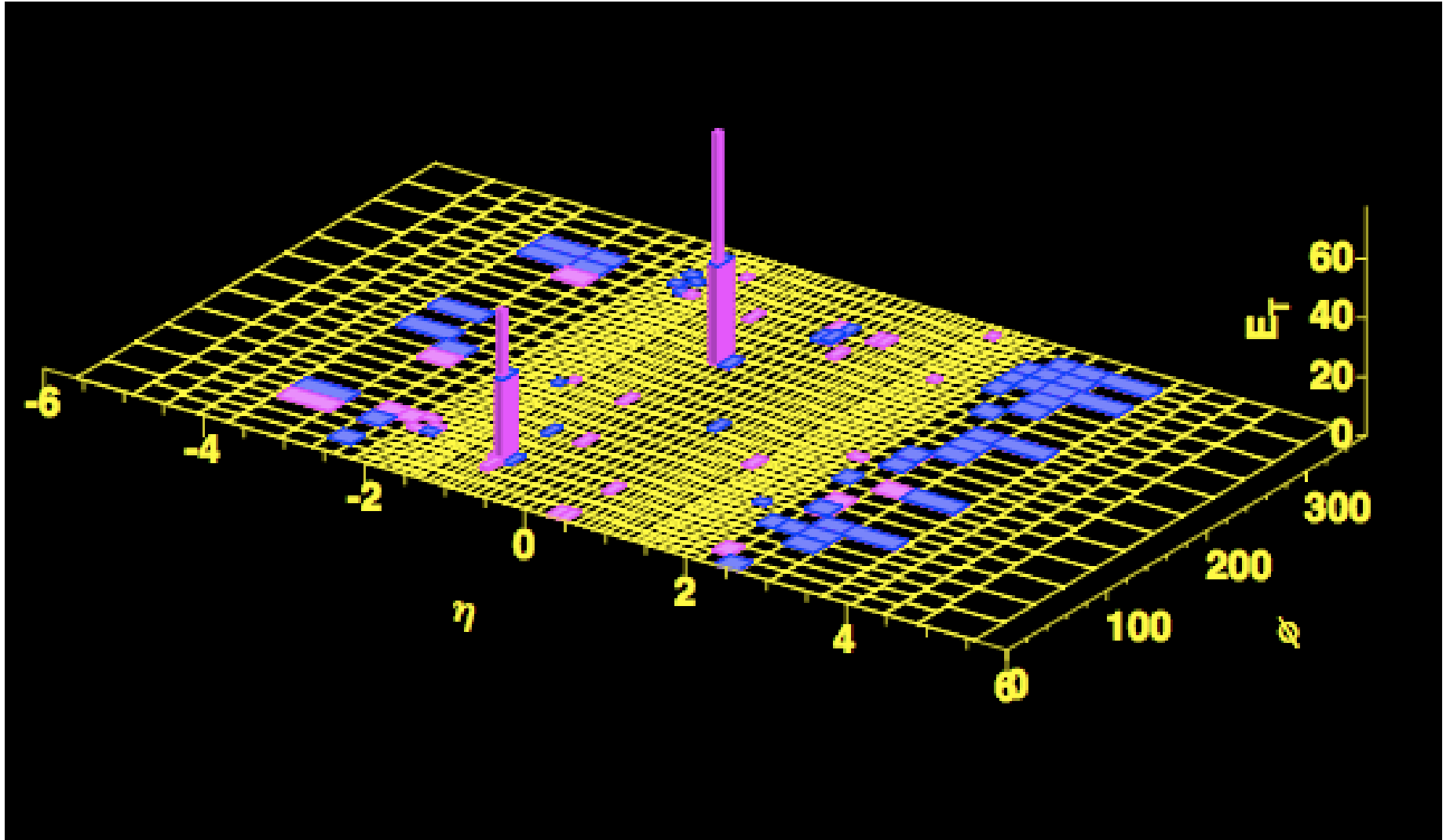
CDF event
