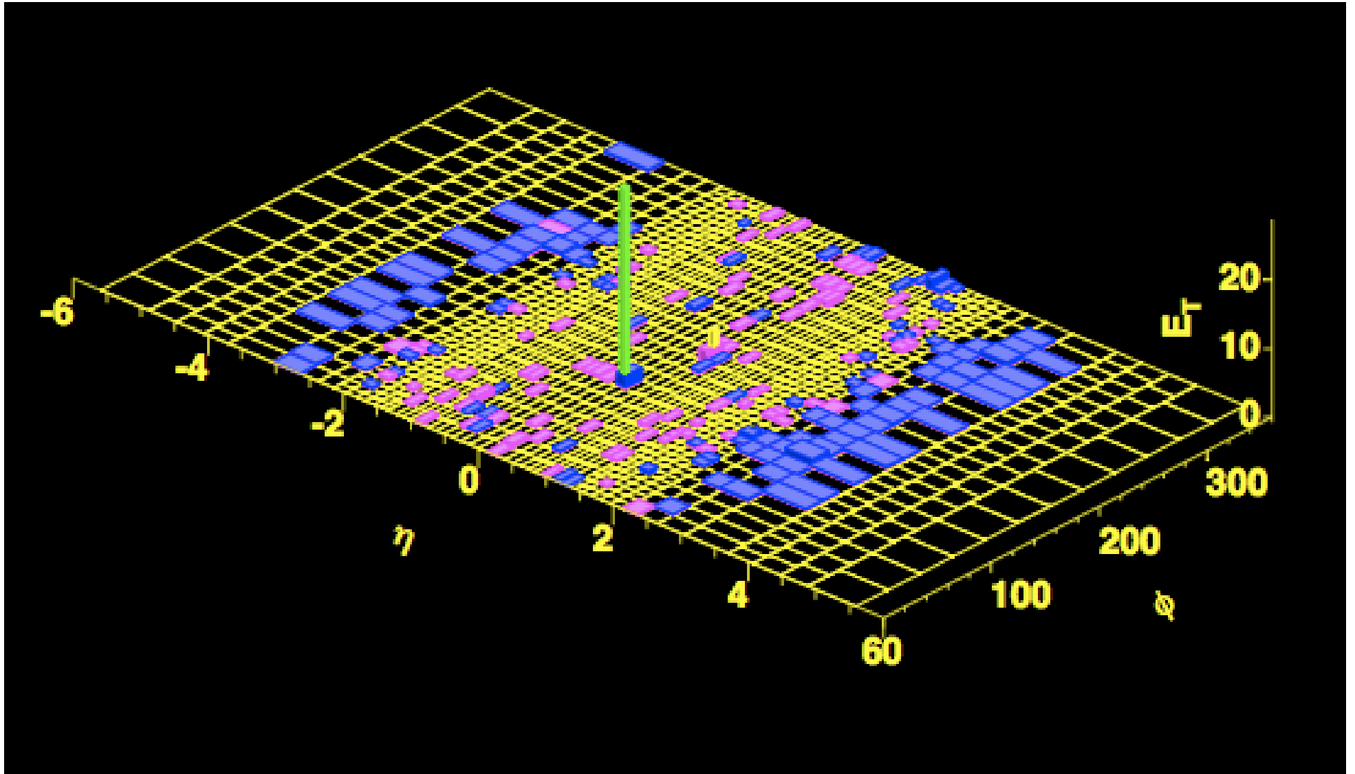
CDF event
